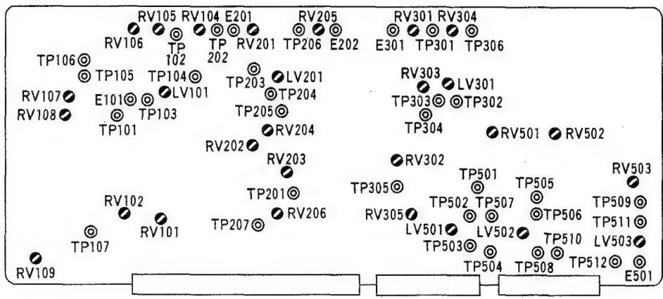
AE-05 board (component side)
